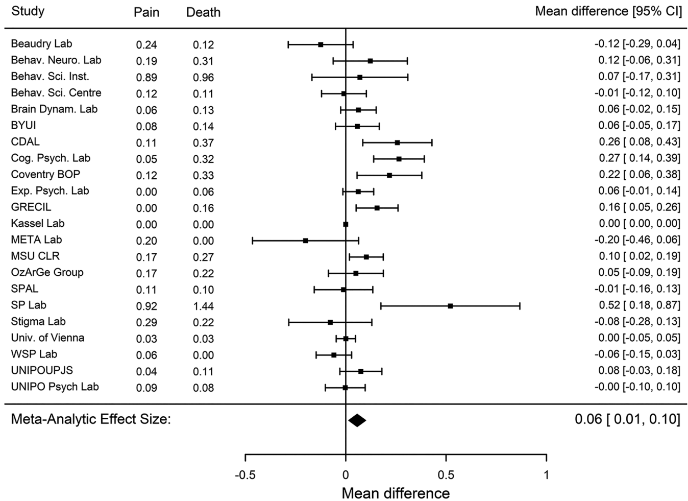
Fig. 4. Forest plot of comparison between death-prime conditions (word-generation task as dependent variable).
